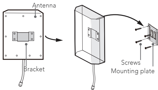
Panel-antenna installation
