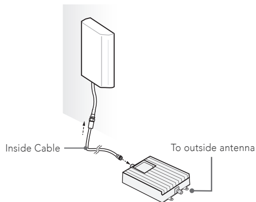
Connecting inside panel antenna to Fusion 5G amplifier
